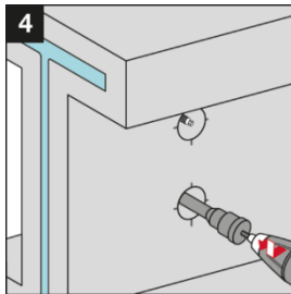
4 Set S-BT studs into drilled hole using the S-DG BT depth gauge.
