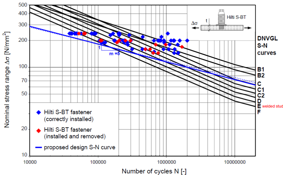
Figure 5: Comparison of Hilti S-BT fatigue test data with DNVGL-RP-C203:2016 fatigue curves and new proposed fatigue curve “S-BT” for Hilti S-BT fastener
