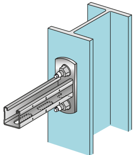
One S-BT stud in each slotted hole
