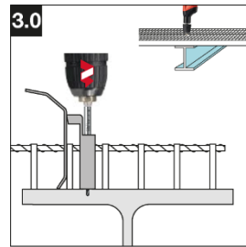
3.0 Pre-drill with TS-BT 5.5-110 S stepped drill bit and S-CS NG centering spacer.
