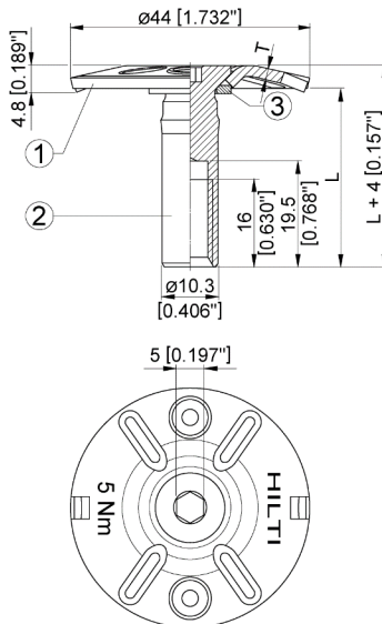
X-FCM-M NG, X-FCM-R NG grating disc
