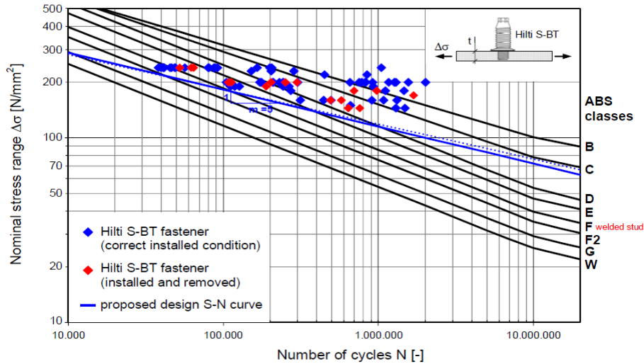
Figure 3: Comparison of Hilti S-BT fatigue test data with ABS-(A) Offshore S-N curves and new proposed fatigue class “S-BT” for Hilti S-BT fastener
