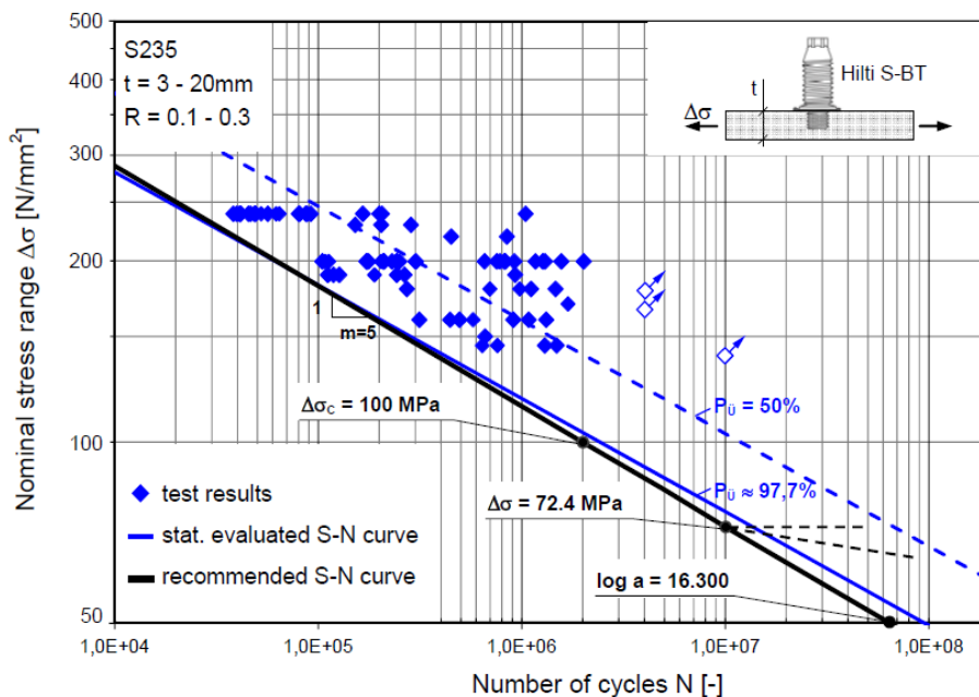
Figure 1: Statistical evaluation of all test results
