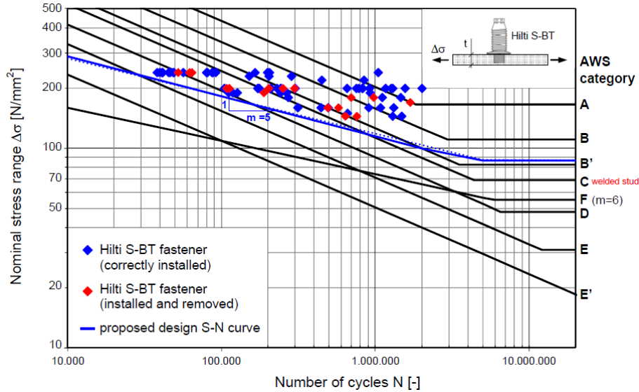
Figure 2: Comparison of Hilti S-BT fatigue test data with AWS D1.1/D1.1M:2015 fatigue categories and new proposed fatigue stress category “S-BT” for Hilti S-BT fastener
