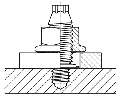
Section of S-BT fastener installed in a pilot hole
