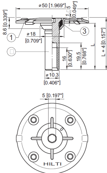
X-FCM, X-FCM-M, X-FCM-R grating discs
