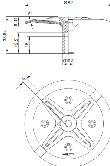
X-FCM-M_L grating disc
