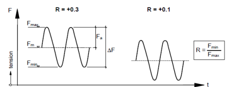
Loading condition of test specimens
