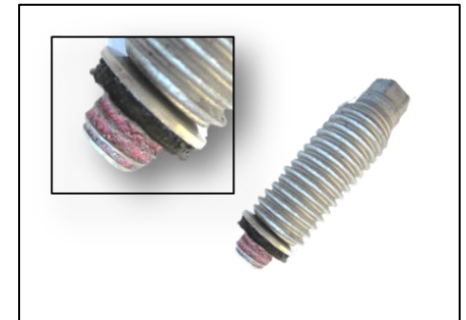
Micro encapsulation on the tapping thread of the S-BT fastener
