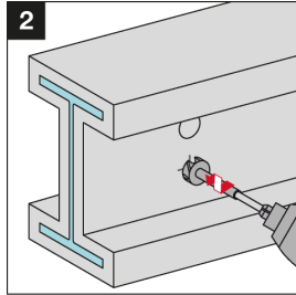
2 Remove PFP and pre-drill with TS-BT 31-74 PFP stepped drill bit ...
