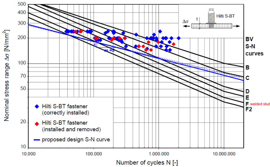
Figure 4: Comparison of Hilti S-BT fatigue test data with BV:2016 fatigue curves and new proposed fatigue curve “S-BT” for Hilti S-BT fastener
