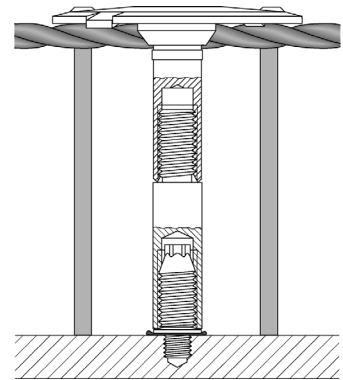
X-SEA-R 30 M8 extension adaptor
