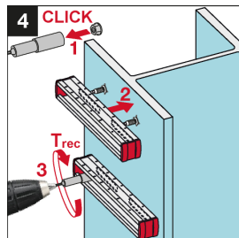
4 CLICK Position channel on S-BT studs and hold in place. Tighten the nuts with the suited installation torque.
