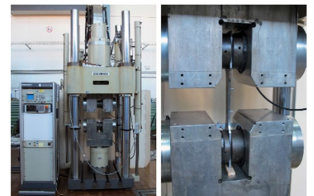
Test facility for fatigue tests
