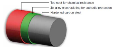
Duplex-coating on carbon steel S-BT fasteners
