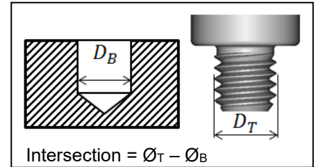
Definition of the thread
